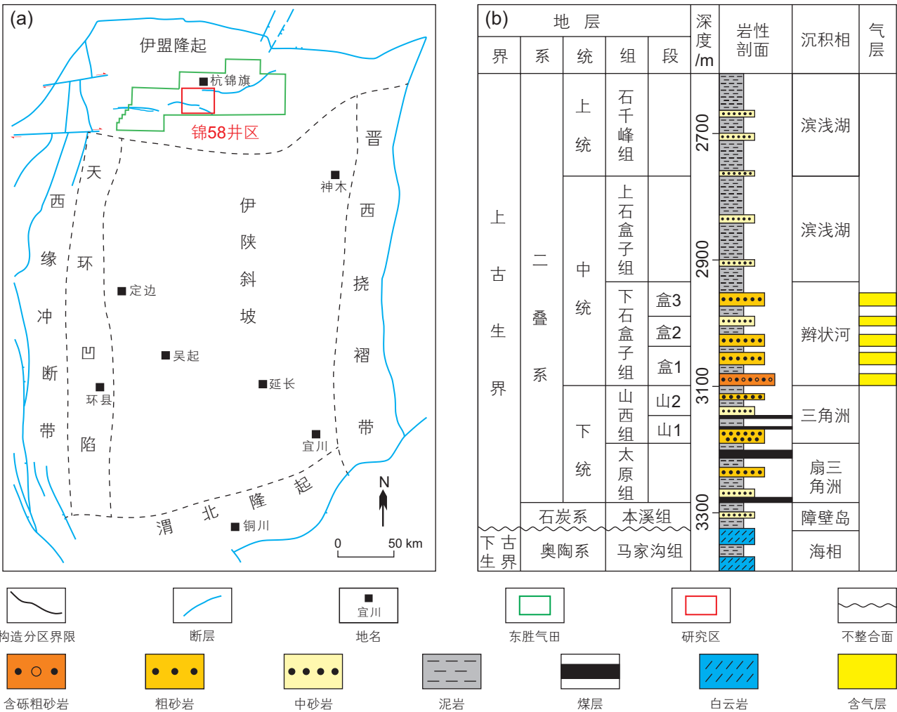
图 1 研究区构造位置(a)及地层综合柱状图(b) Fig. 1 Tectonic location (a) and comprehensive stratigraphic histogram (b) of the study area
